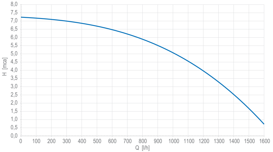
fig. 59- Residual head available for system
